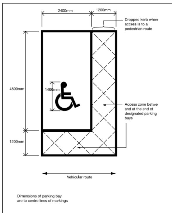
Diagram 2 – Parking bay designated for disabled people
