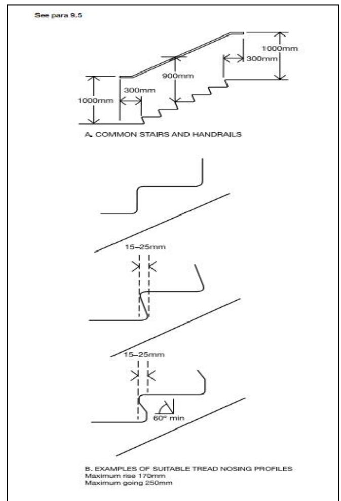
Diagram 30 Common stairs in blocks of flats
