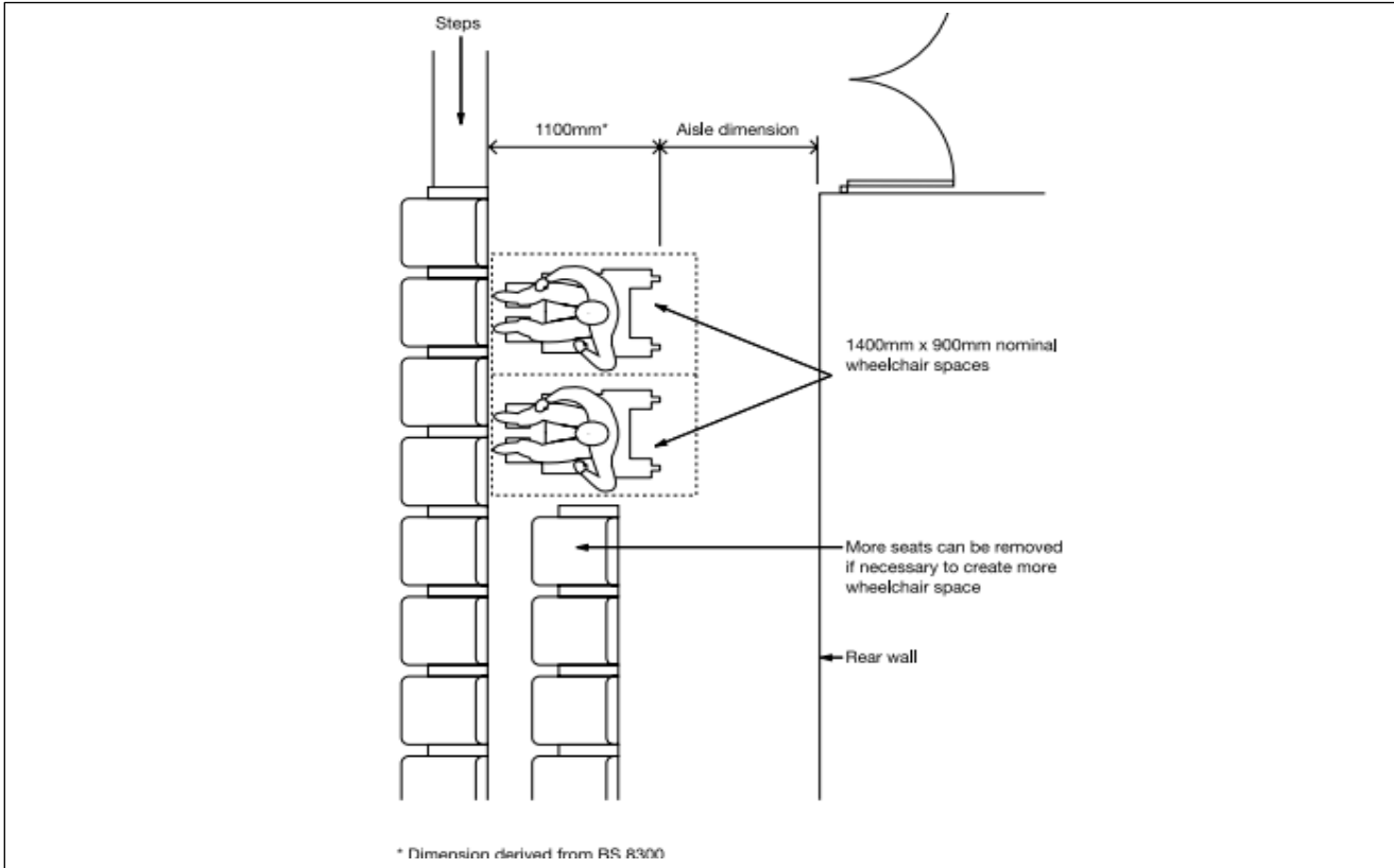
Diagram 15 An example of wheelchair space provision in a cinema or theatre
