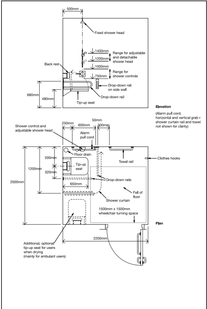
Diagram 23 An example of a self-contained shower room for individual use
