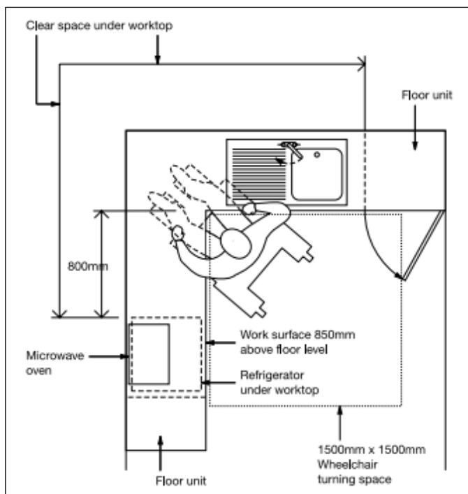
Diagram 16 An example of a shared refreshment facility
