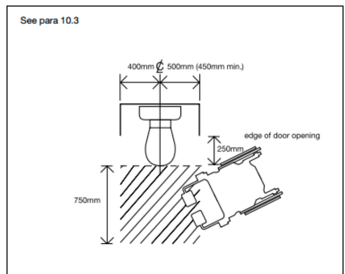
Diagram 32 Clear space for oblique access to WC
