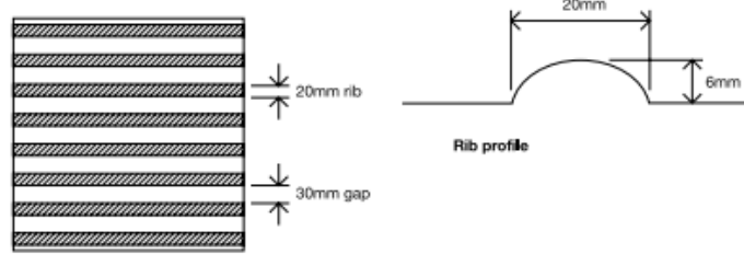
'Corduroy' hazard warning surface (with 8mm ribs)
