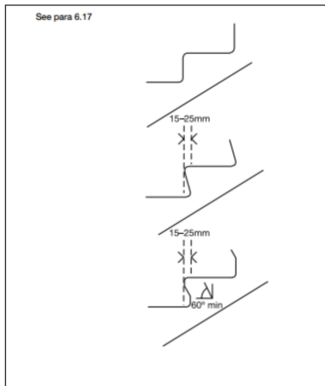
Diagram 27 External Step Profile
