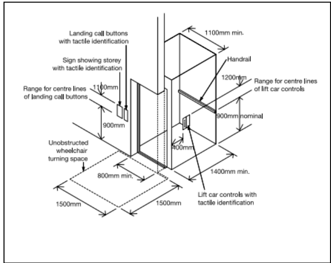
Diagram 11 Key dimensions associated with passenger lifts
