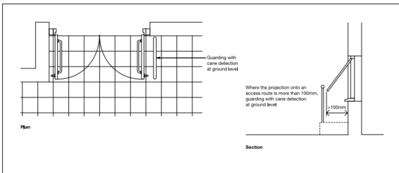
Diagram 8 Avoiding hazards on access routes
