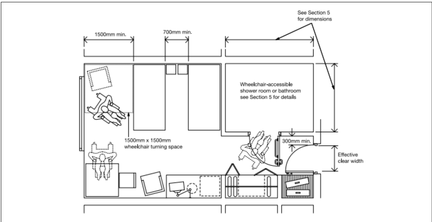
Diagram 17 One example of wheelchair-accessible hotel bedroom with en-suite sanitary facilities
