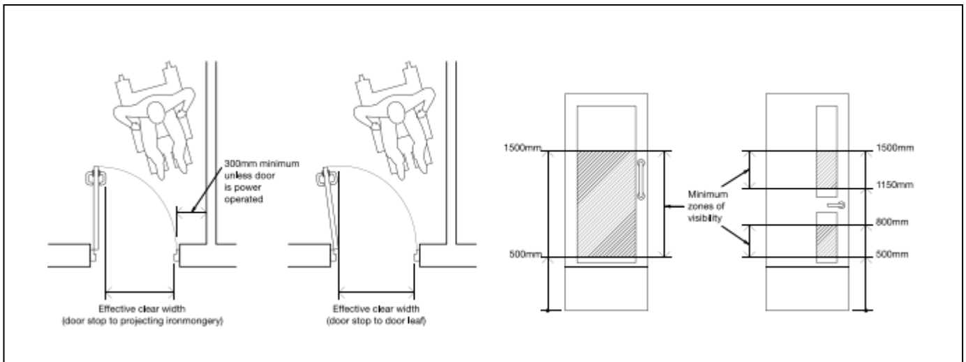
Diagram 9 Effective clear width and visibility requirements of doors
