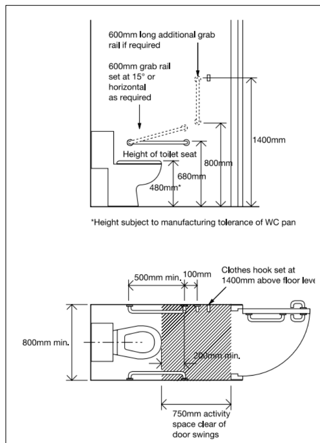
Diagram 21 WC cubicle for ambulant disabled people
