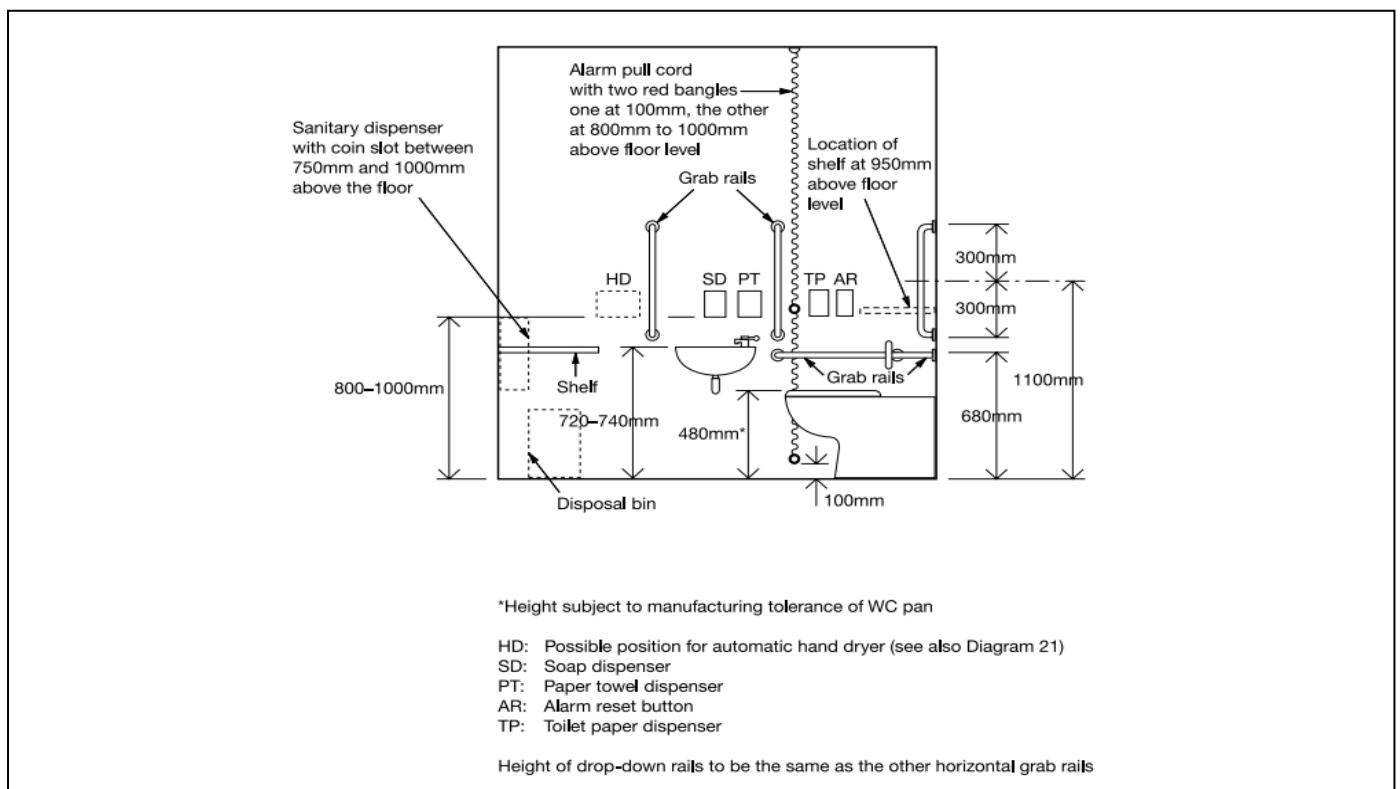
Diagram 19 Heights and arrangement of fittings in a unisex wheelchair-accessible toilet (looking towards wall A in Diagram 18)
